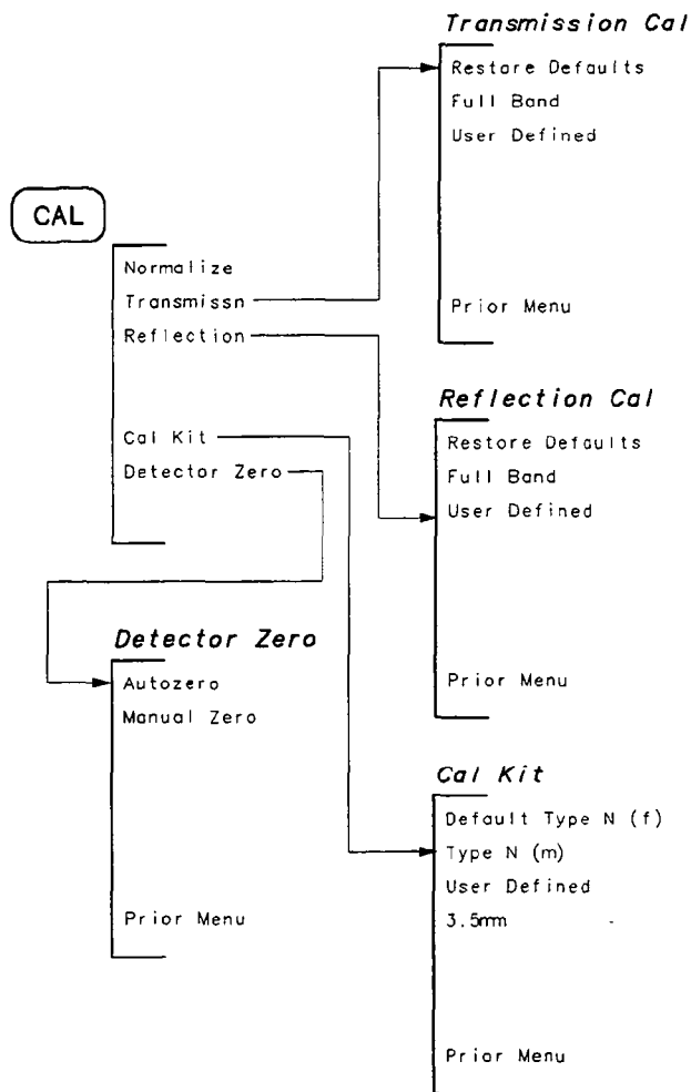
Figure 7-3. Calibration Menu
