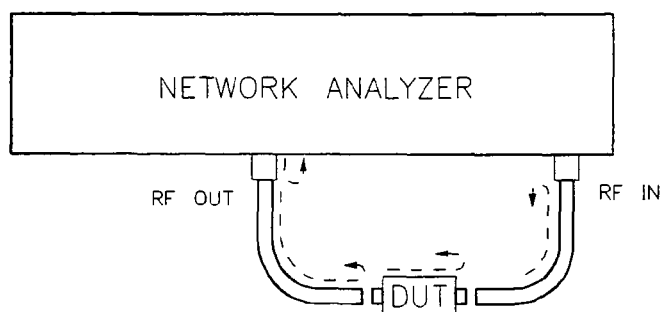
Figure 8-6. Mismatch Errors
