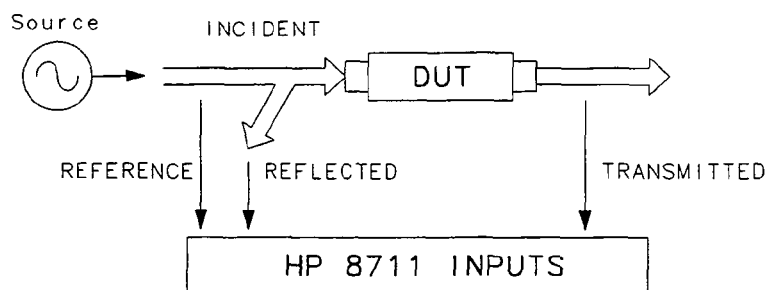
Figure 4-2. Receiver Inputs for Transmitted, Reflected, and Reference Signals
