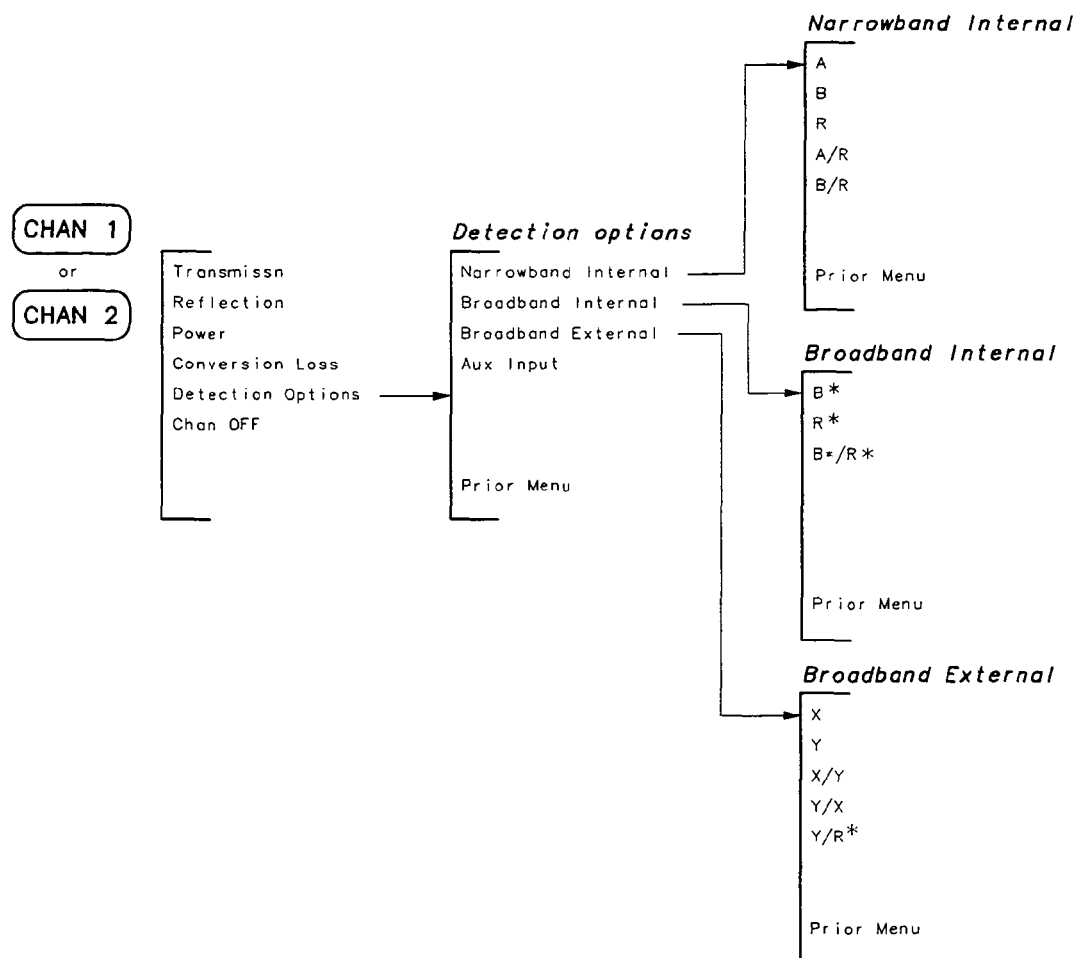
Figure 7-9. Measurement Menu
